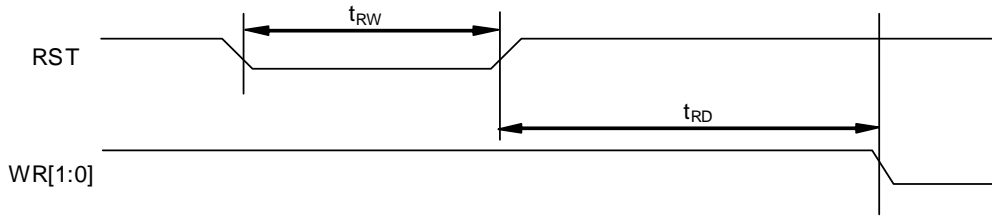
FIGURE 19: Reset Characteristics
