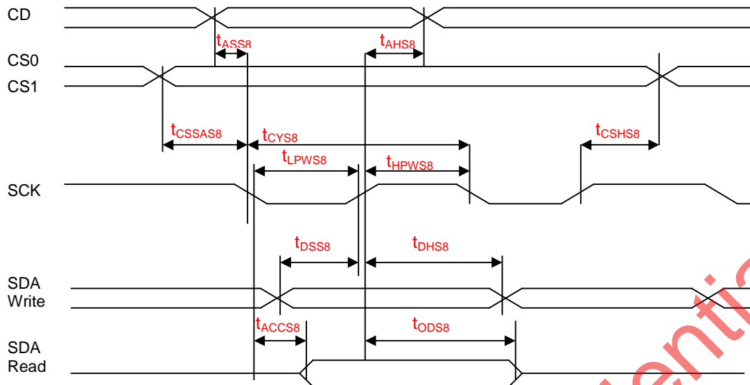
FIGURE 16: Serial Bus Timing Characteristics (for S8)
