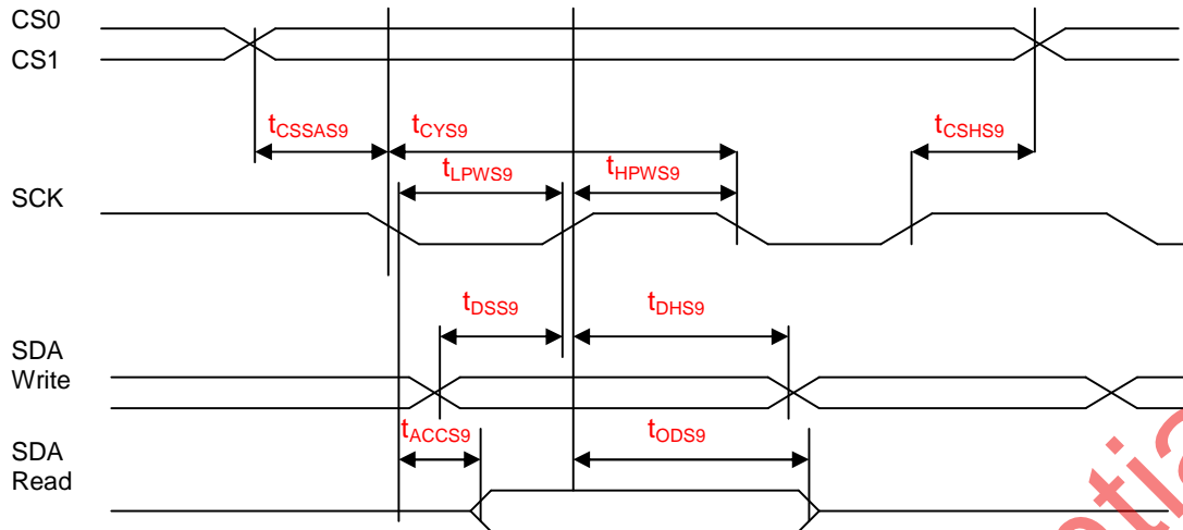
FIGURE 17: Serial Bus Timing Characteristics (for S9)
