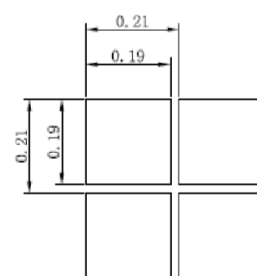
Detail A (30:1)
